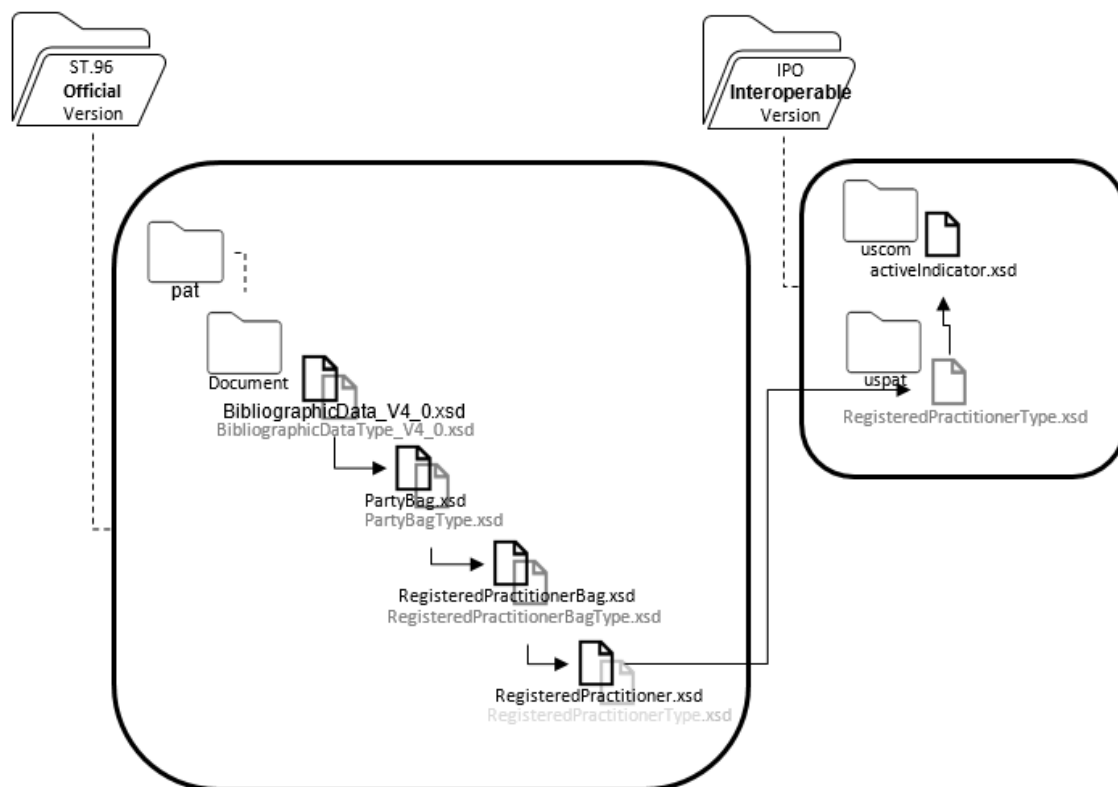
Figure 8: Graphical View
