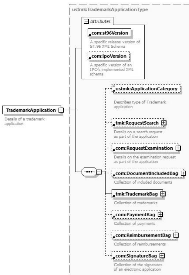
Figure 21: ustmk: TrademarkApplication
