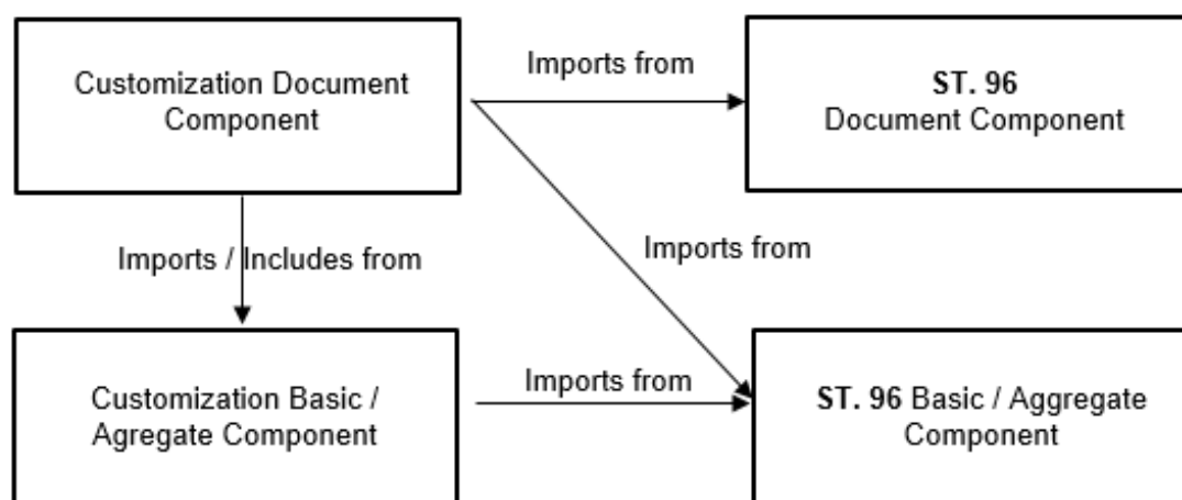
Figure 2: Specifying using both ST.96 and non-ST.96 Components
