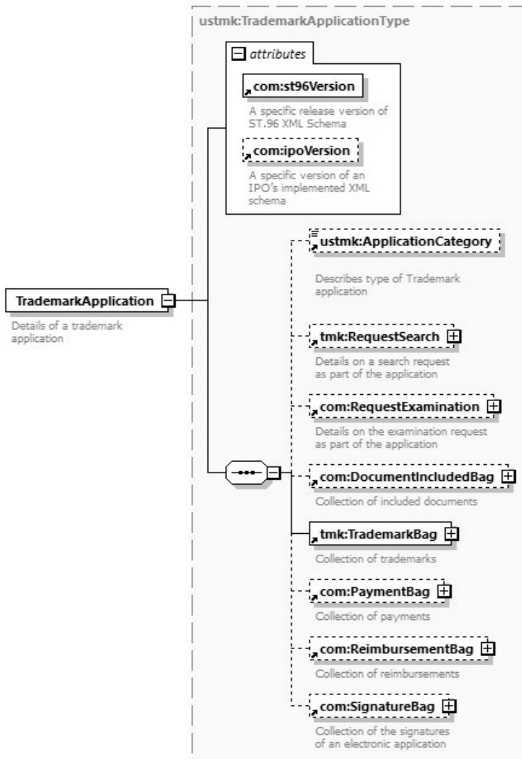
Figure 21: ustmk: TrademarkApplication
