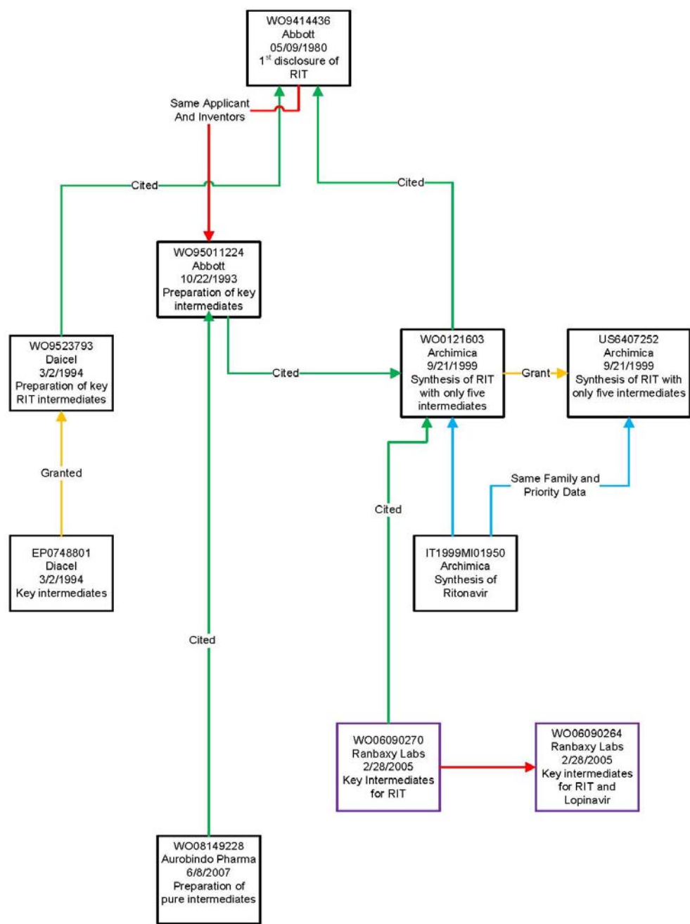
Innovation Track 2- Synthesis of Ritonavir
