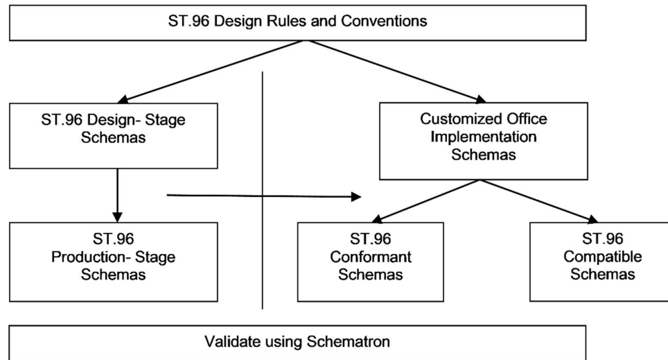
Figure 3: Overview of ST.96 customization process
