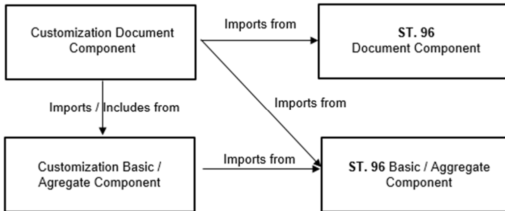
Figure 2: Specifying using both ST.96 and non-ST.96 Components
